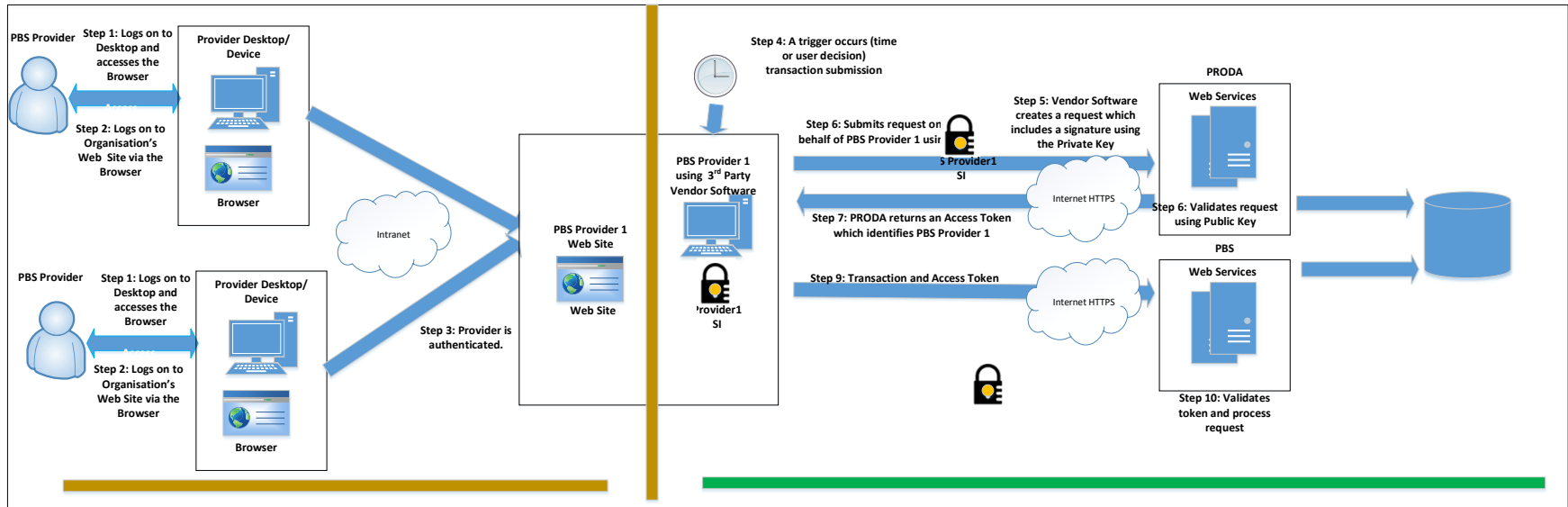
Unattended Scenario using on-premise configuration to authenticate and submit unattended transaction for PBS Provider 1
